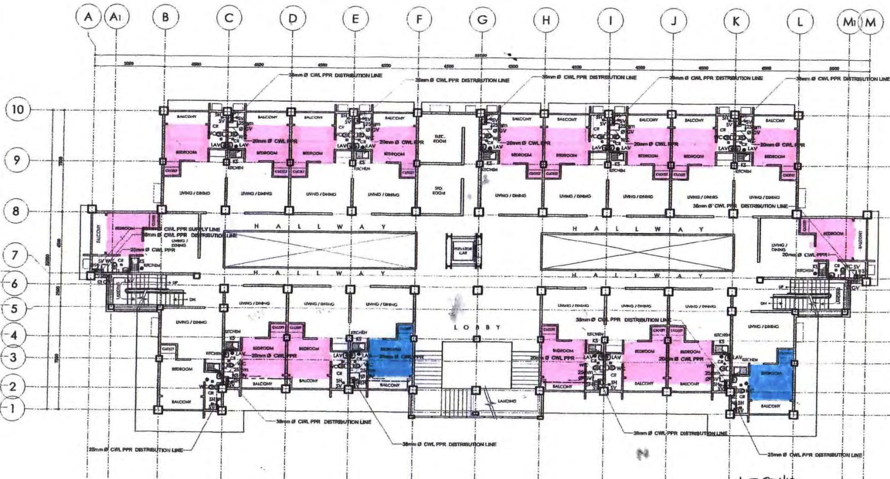
TYPICAL SECOND AND THIRD FLOOR WATER LINE LAYOUT SCALE 1 : 100 MTS.
