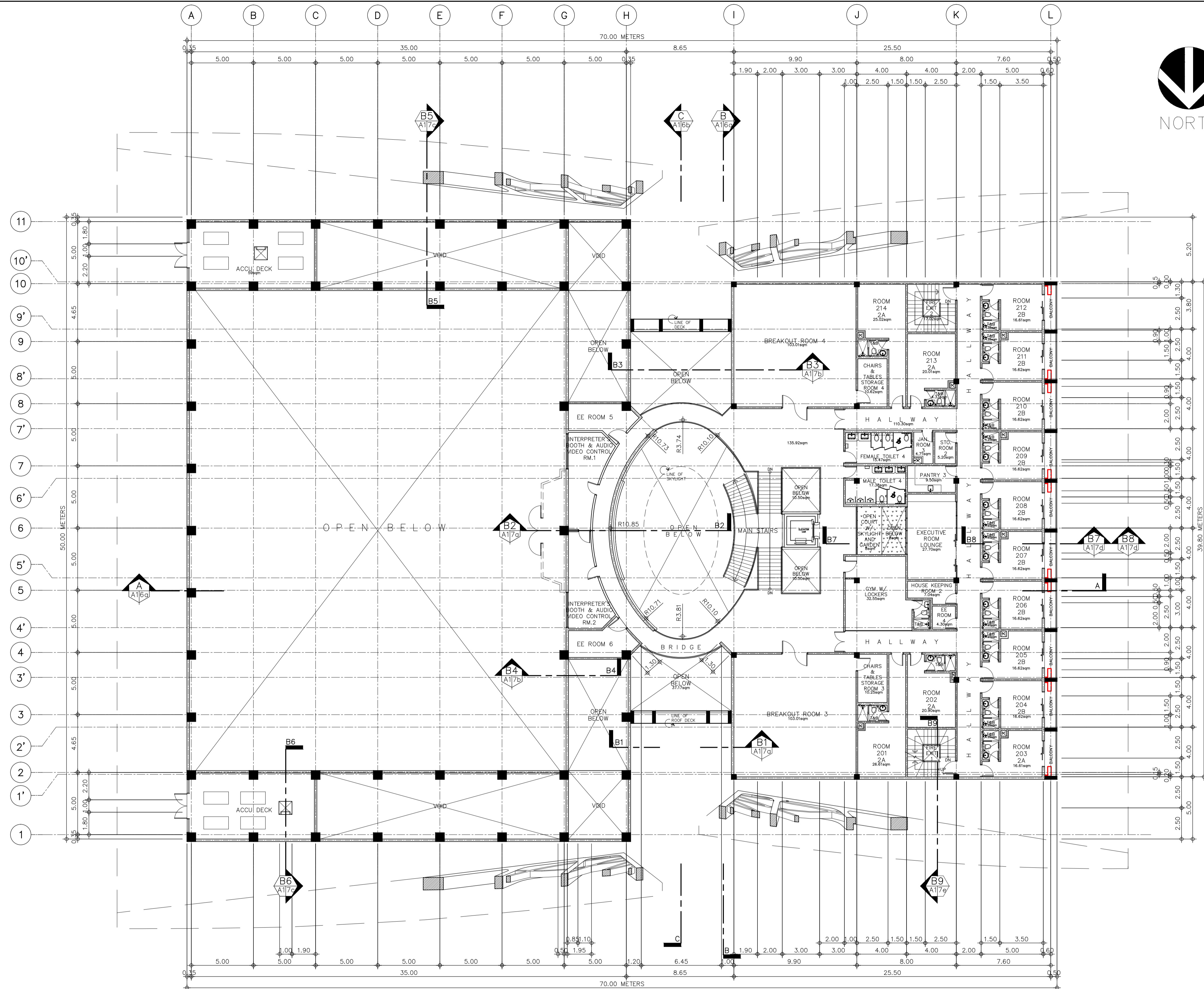
A SECOND FLOOR PLAN SCALE 1:175M
