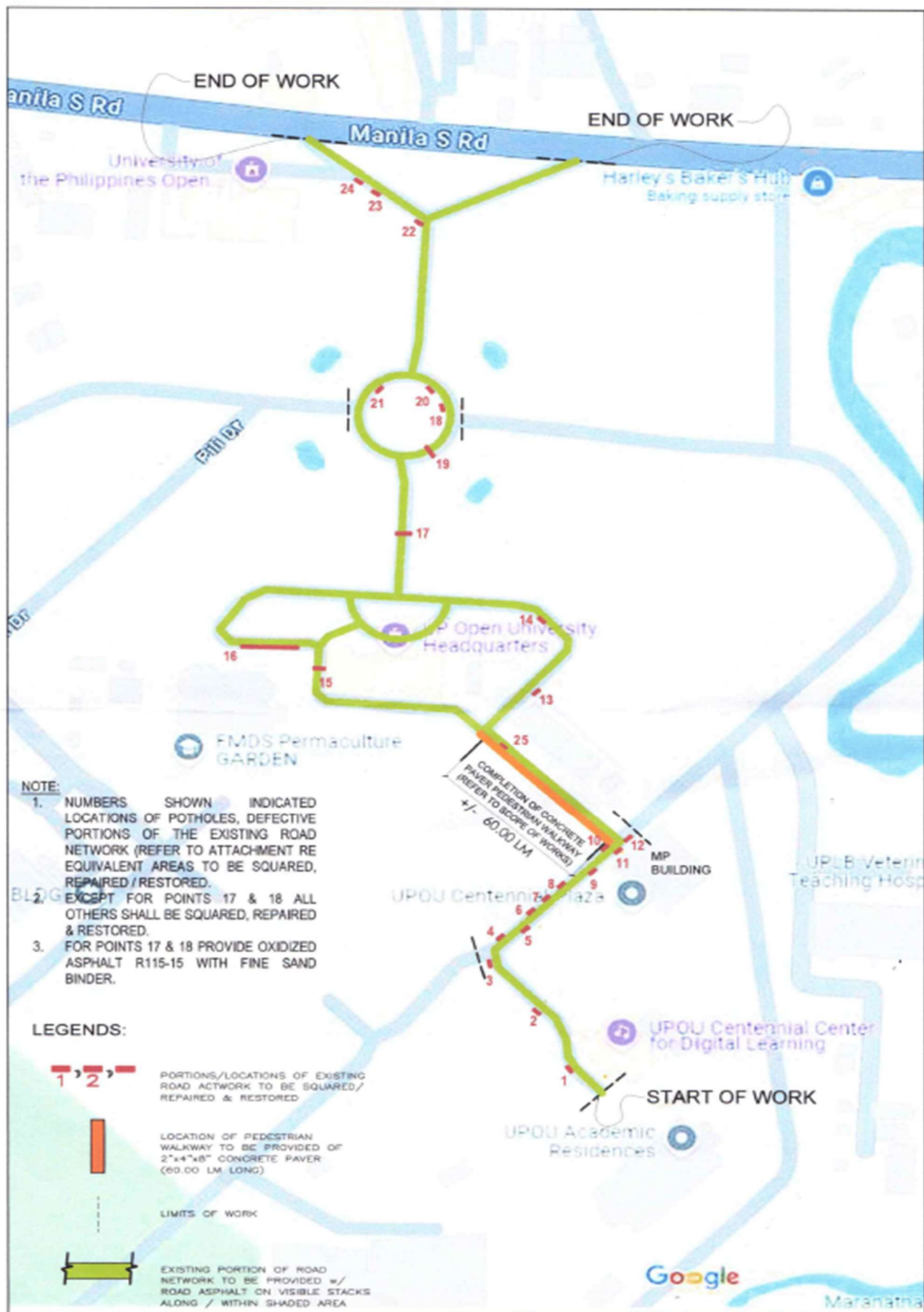
A PLAN (EXISTING UPOU ROAD NETWORK) A-01 NOT TO SCALE
