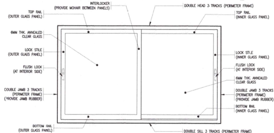
ALUMINUM PARTS SHALL BE 900 SERIES POWDER COATED WHITE 6063-T5 ALUMINUM
