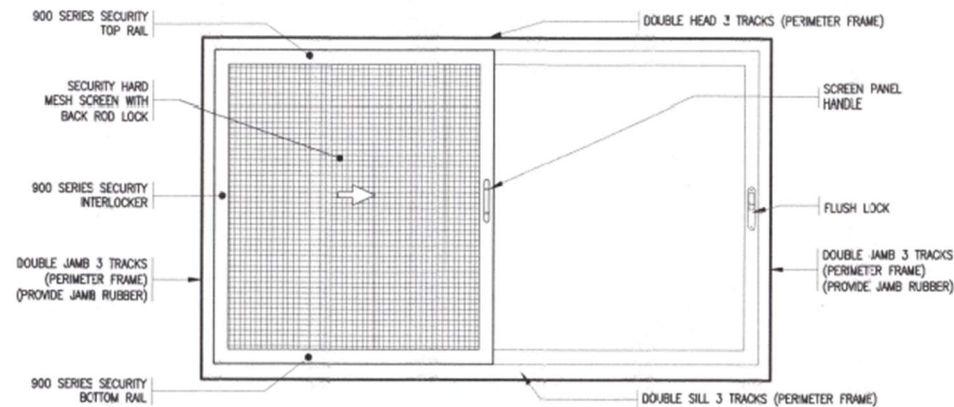
ALUMINUM PARTS SHALL BE 900 SERIES POWDER COATED WHITE 6063-T5 ALUMINUM TYPICAL PARTS IDENTIFICATION - SCREEN PANEL (INTERIOR)
